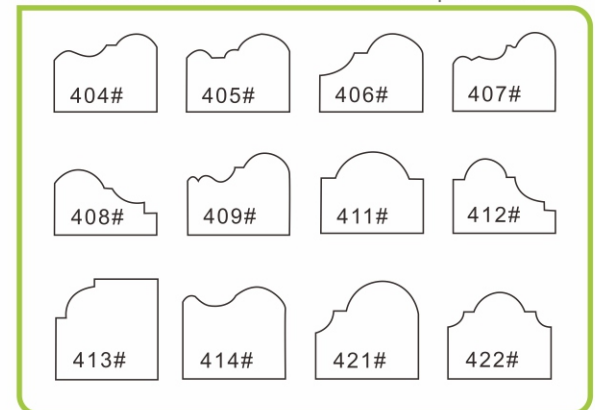
4公分系列电镀轮 4cm series electroplated wheels
